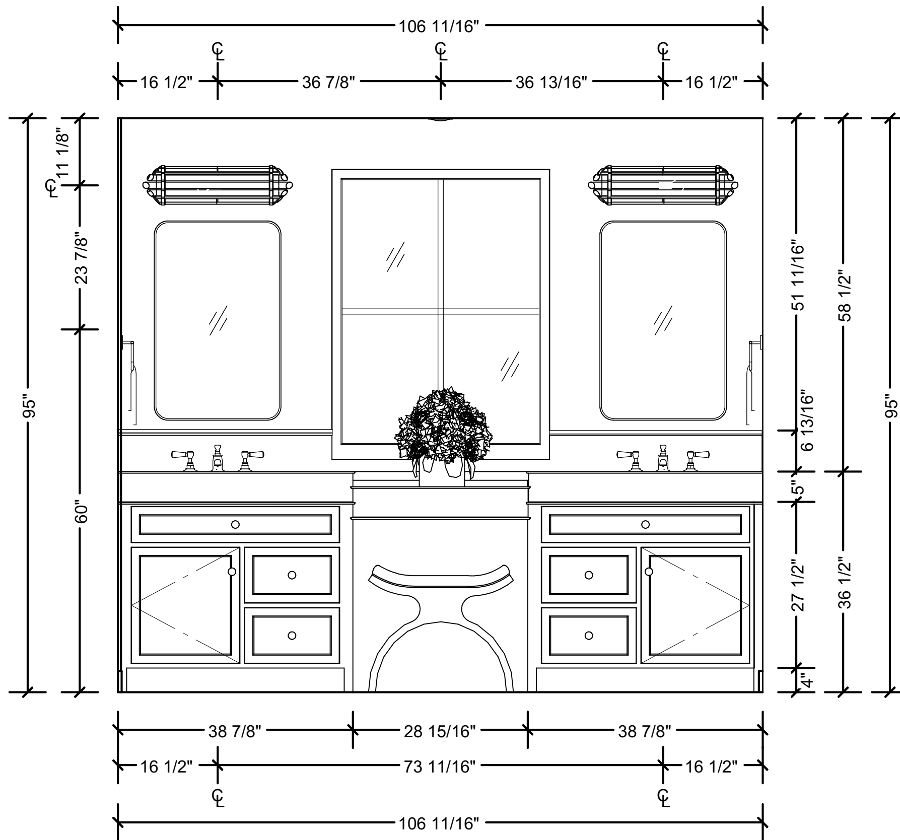
Primary Bath Elevation 1 3/4 in = 1 ft
