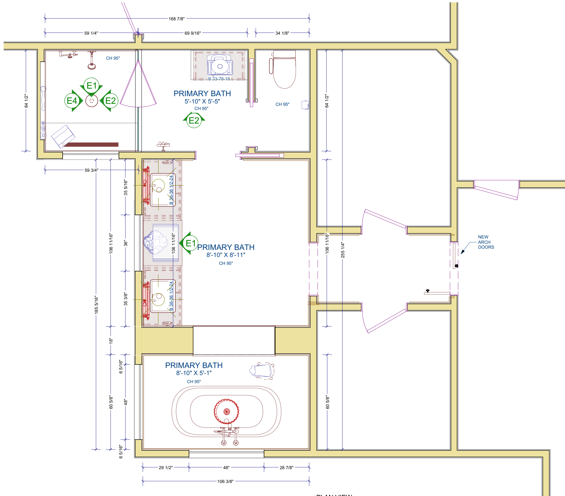
PLAN VIEW 3/8 in = 1 ft
