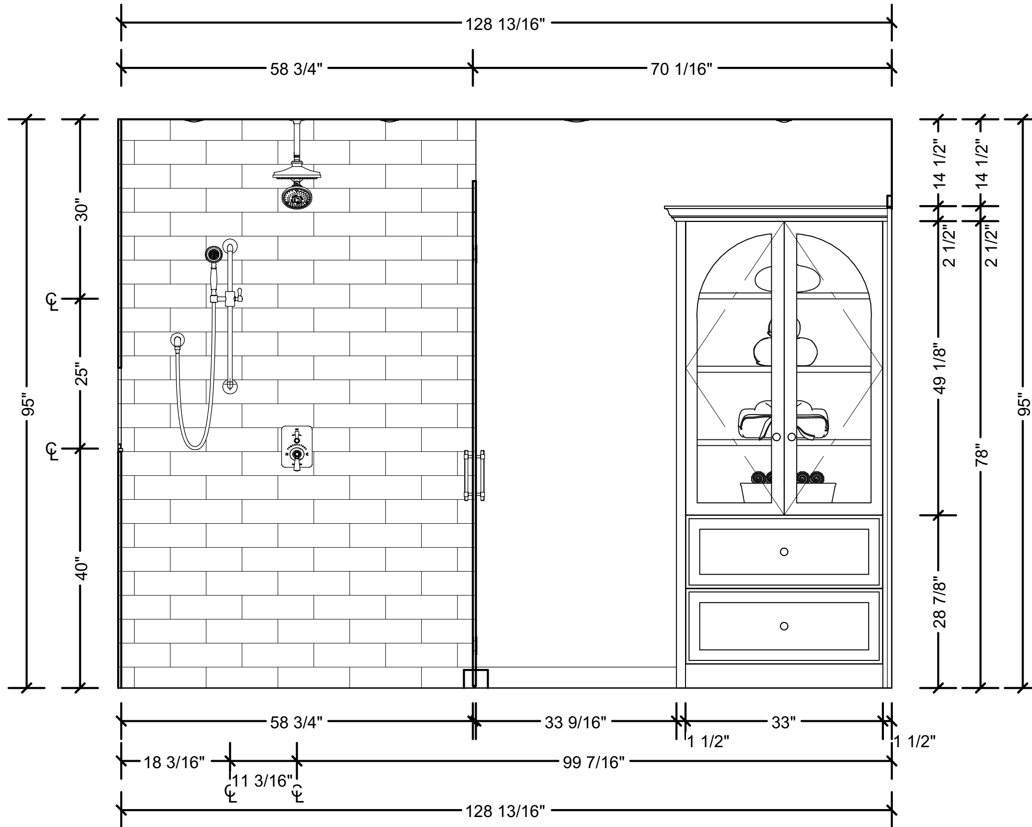
Primary Bath Elevation 2 3/4 in = 1 ft
