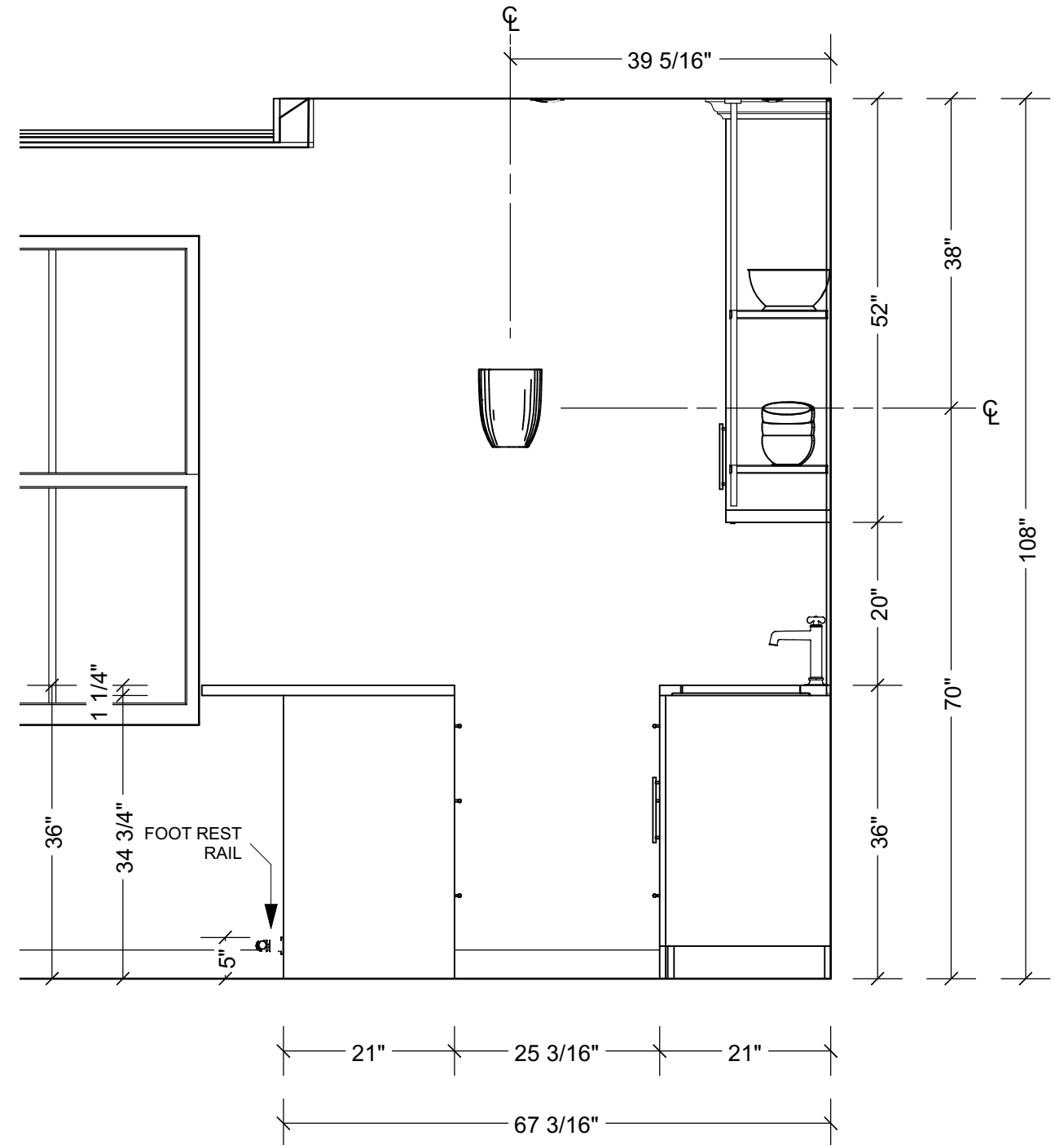
Bar Elevation 3 5/8 in = 1 ft
