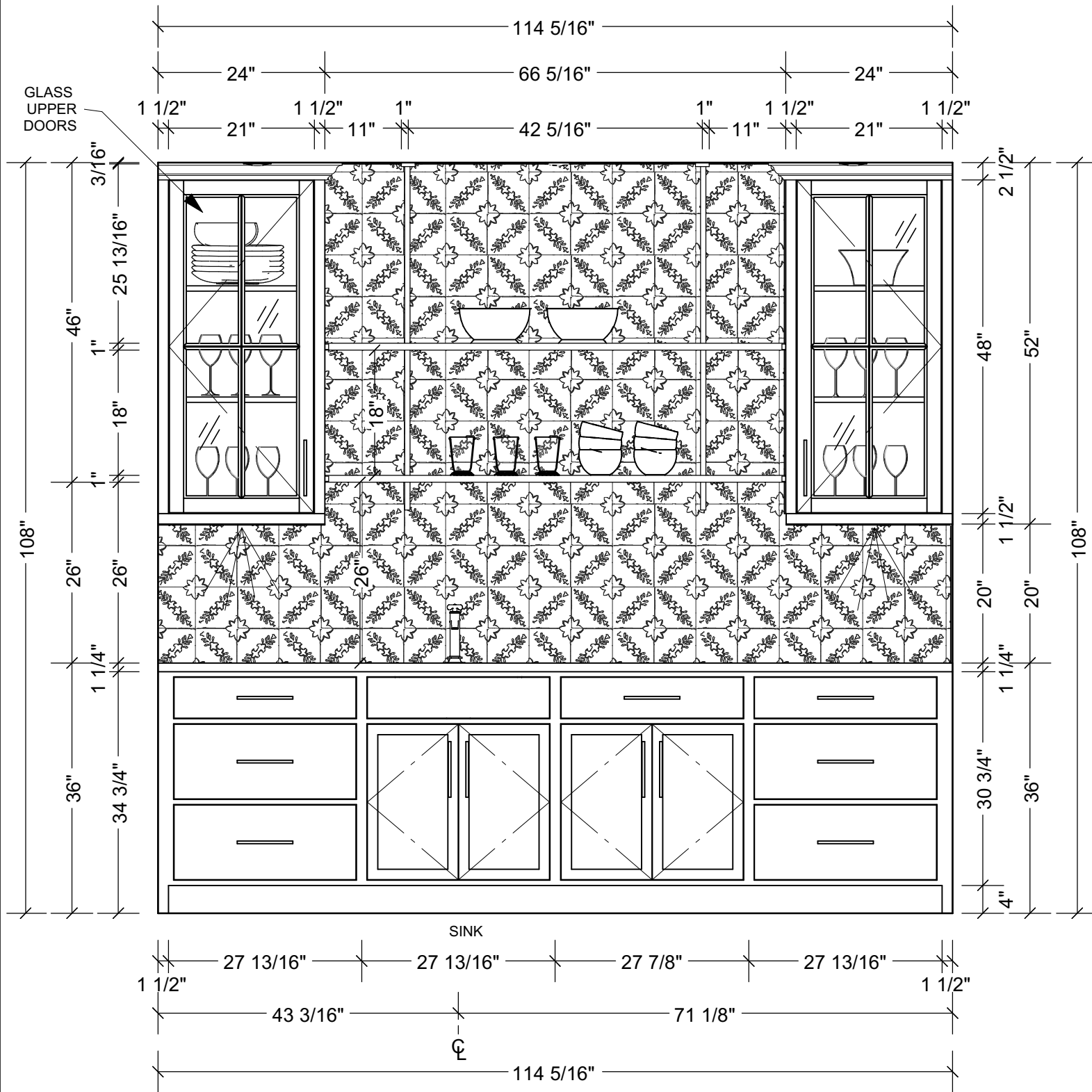
Bar Elevation 1 5/8 in = 1 ft
