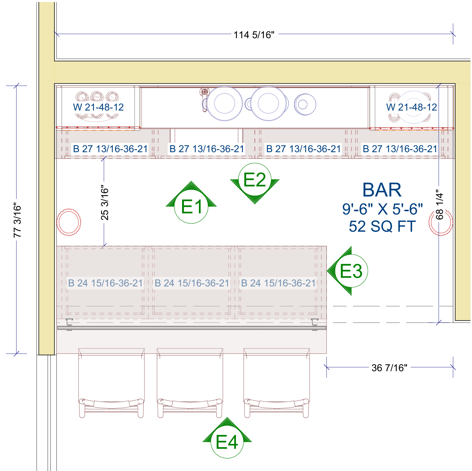
BAR PLAN VIEW 3/4 in = 1 ft
