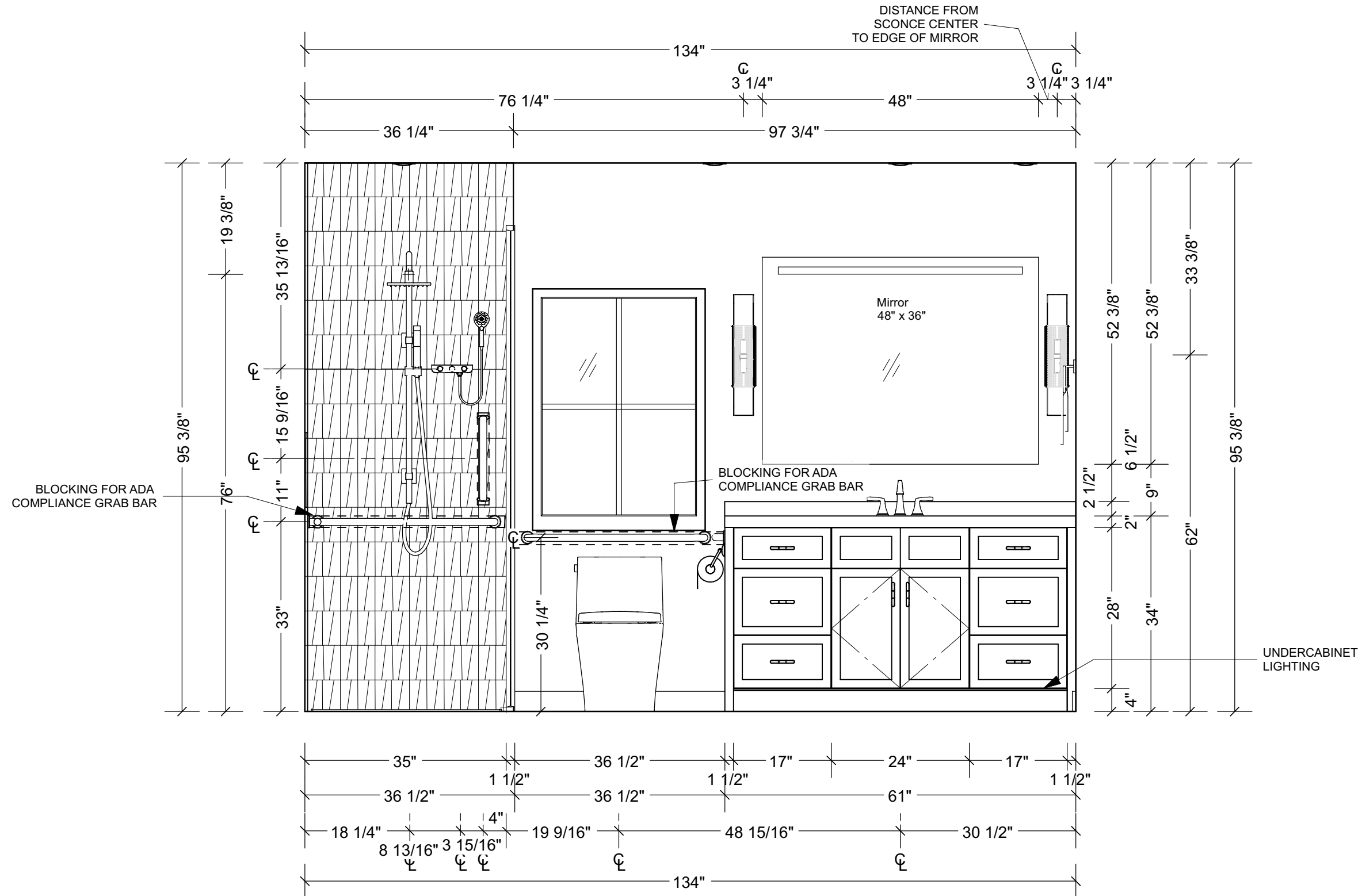
MIL Suite Bath Elevation 1 5/8 in = 1 ft
