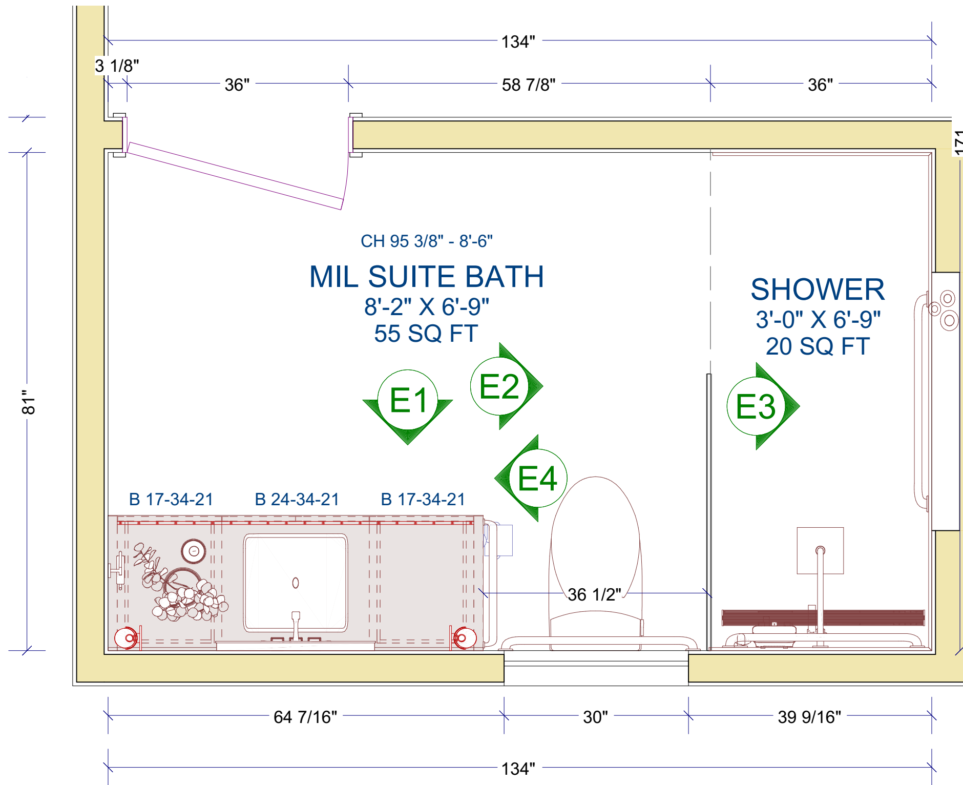
PLAN VIEW 3/4 in = 1 ft
